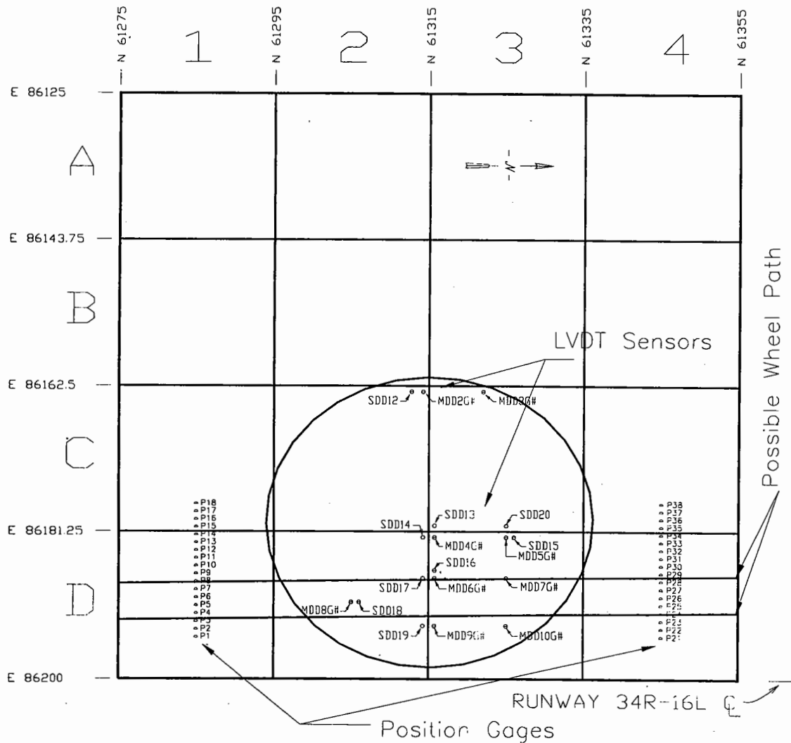
a) Location of the LVDT sensors
