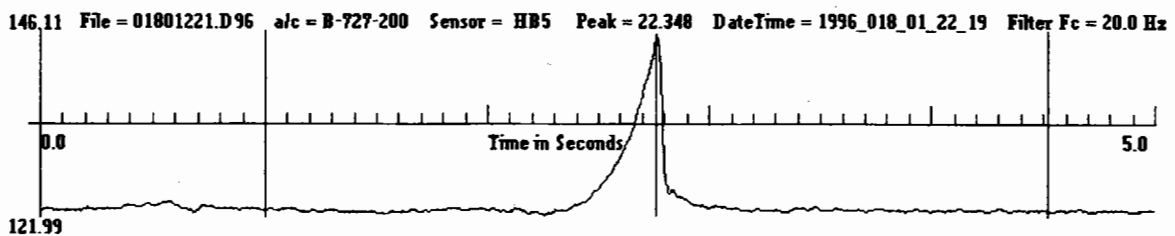
b Transverse strain at transverse edge for B-727
